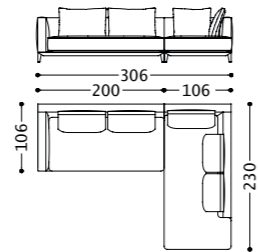
01BOWC2 (1BOW210SX + 1BOW260DX) 02BOWC2 (2BOW210SX + 2BOW260DX)
