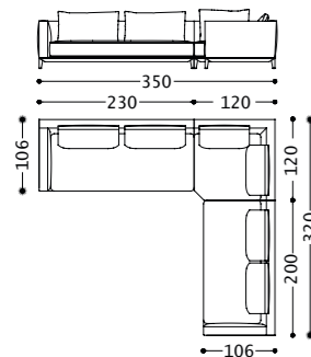
01BOWC7 (1BOW220SX + 1BOW300 + 1BOW210DX) 02BOWC7 (2BOW220SX + 2BOW300 + 2BOW210DX)
